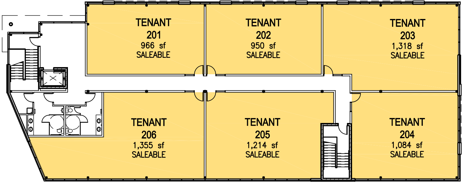
SECOND FLOOR
